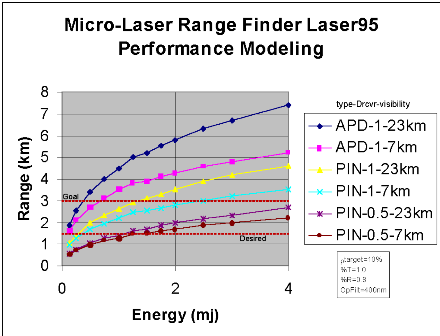
Figure 6. Modeled performance for the m LRF.
