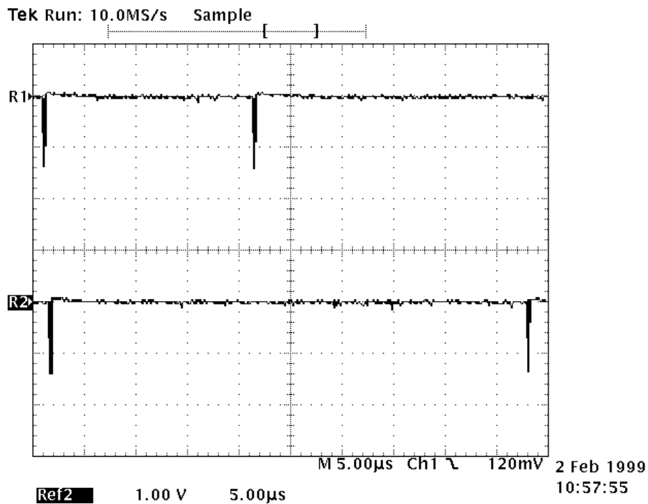
Figure 13. mLRF START and STOP signals on scope display.
