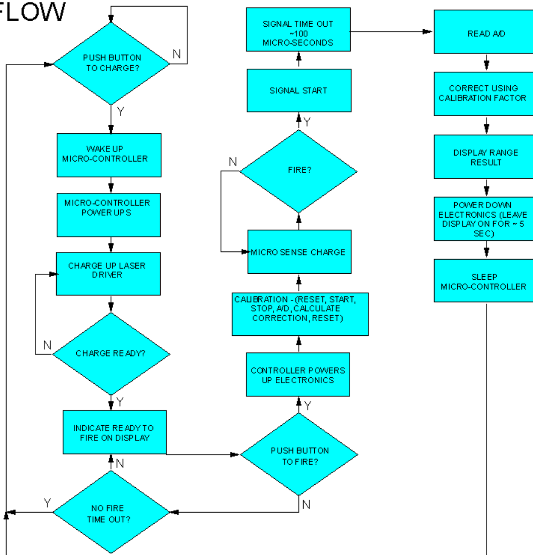
FIGURE 4. mLRF system control logic flow diagram.
