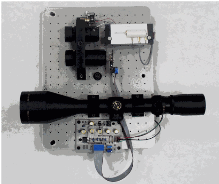
Figure 14. mLRF Laboratory Prototype.
