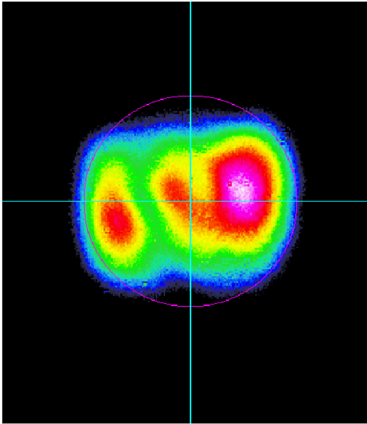
Raw Beam (8 mRad aperture)
