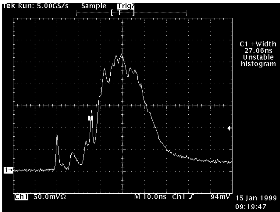
Figure 9. Pulse width measurement of the Monolithic Laser Cavity (MLC)
