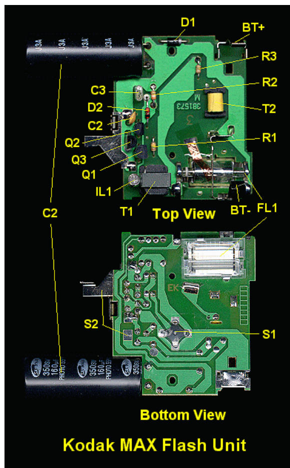
Figure 5. Circuit from a Kodak MAX flash camera
